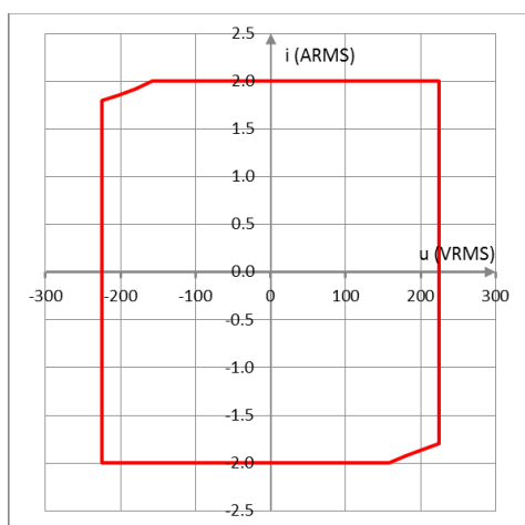
RANGE 225V
